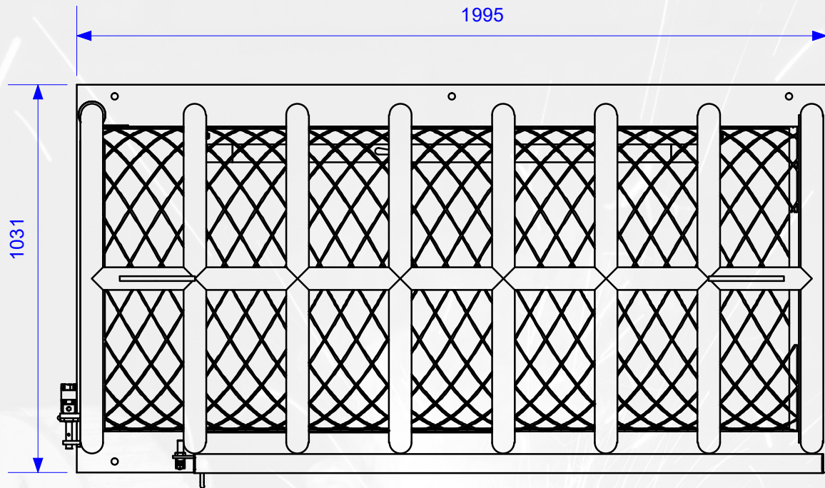
VISTA CENITAL
